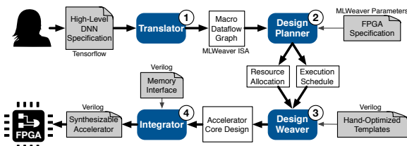
Figure 1: Overview of MLWEAVER which takes a high-level specification of the DNN and the target FPGA to generate the accelerator design as synthesizable Verilog along with the accelerator execution schedule and the layout of the DNN model in the memory.
